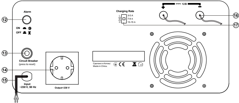
Fig. 3. Rear panel of RT-500
