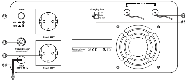
Fig. 4. Rear panel of RT-1000
